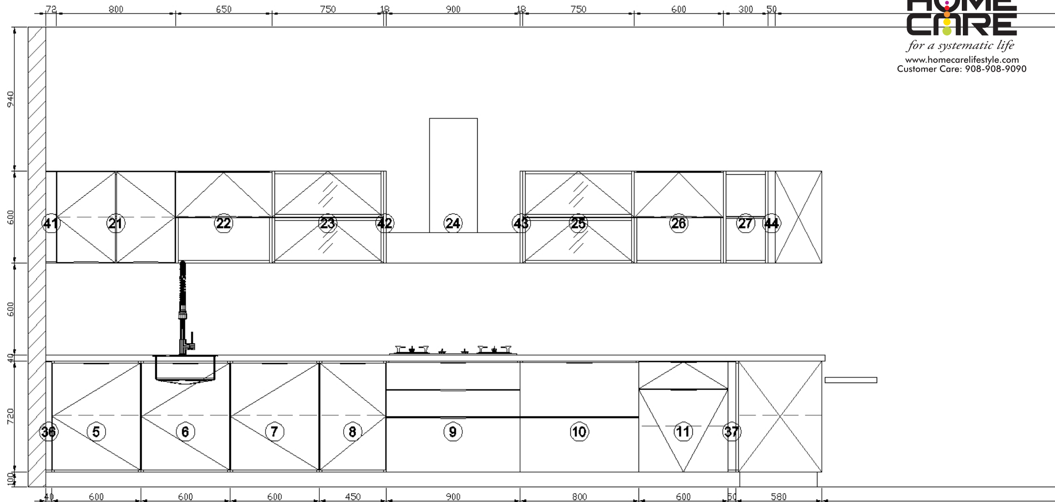
B View elevation drawing
